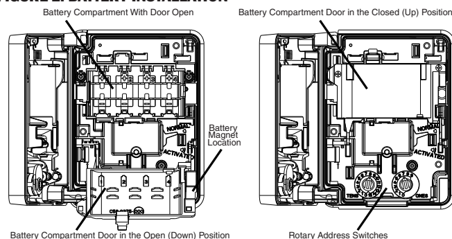
FIGURE 2. BATTERY INSTALLATION
