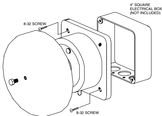
Figure 3. Surface installation:
