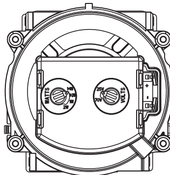
Figure 6 Speaker Wattage and Voltage Settings
