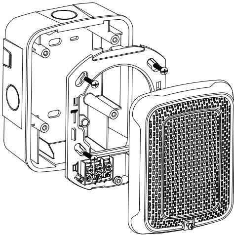
FIGURE 7. SURFACE MOUNTING ON WALL (SBBSPRL, SBBSPWL)
