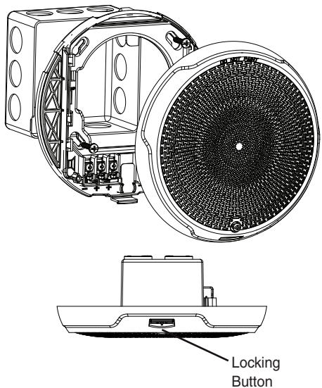
FIGURE 5. CEILING SPEAKER
