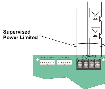
Figure 5: Class A (Style Z) Speaker Configuration
