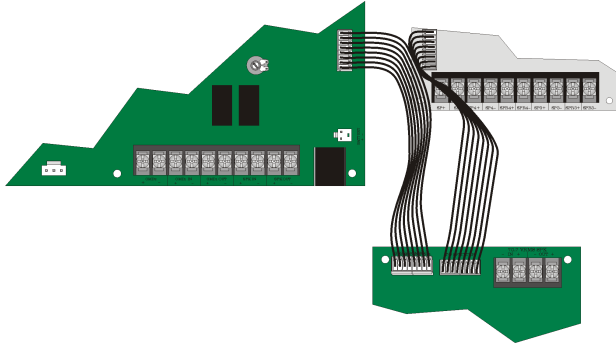
Figure 3: Wire Harness Connection From the Main Control to the SKE-V70
