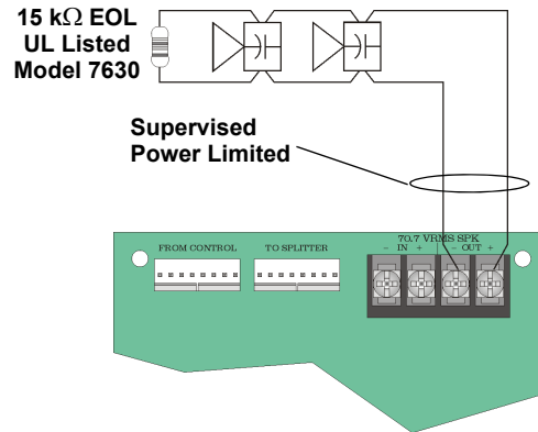
Figure 4: Class B (Style Y) Speaker Configuration
