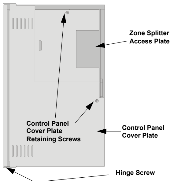
Figure 1: View of Cabinet With Cover Plate in Place
