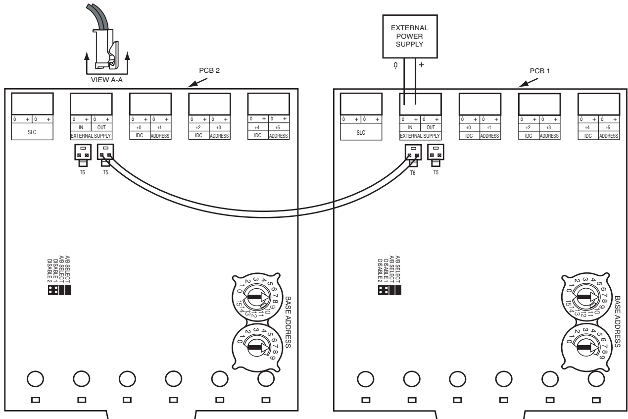
FIGURE 8. EXAMPLE OF MULTIPLE BOARDS SHARING SAME EXTERNAL SUPPLY
