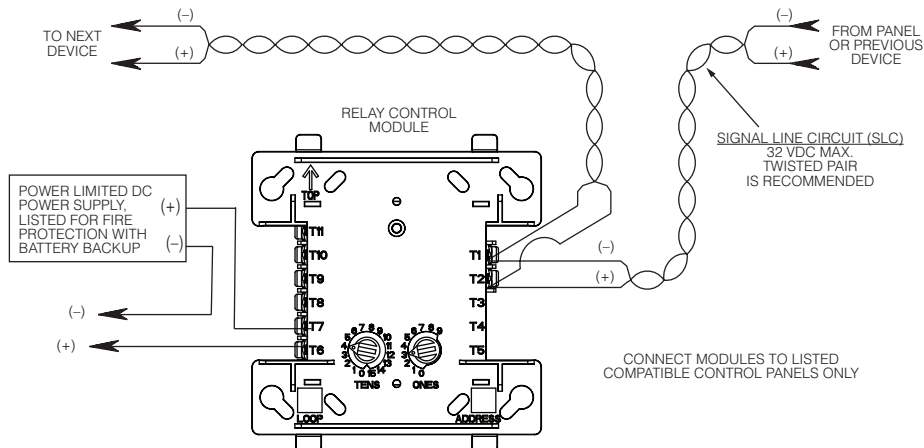
FIGURE 7. RELAY CONTROL MODULE USED TO DISCONNECT A POWER SUPPLY
