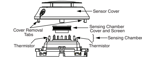
FIGURE 4: CLEANING THE PHOTO/HEAT DETECTOR
