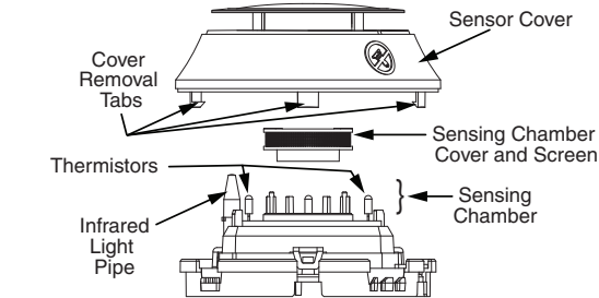
FIGURE 4. CLEANING THE FIRE/CO DETECTOR
