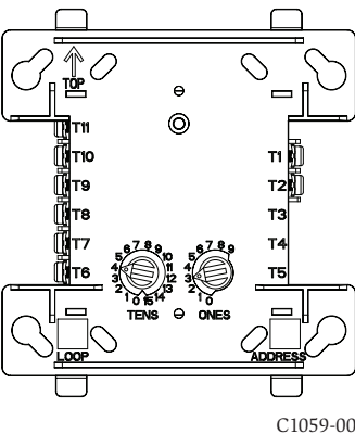
FIGURE 1A. CONTROLS AND INDICATORS:
