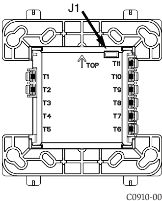
FIGURE 1B. JUMPER LOCATION:
