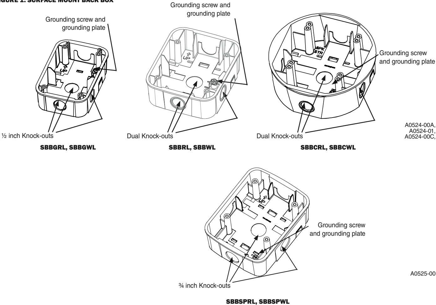
FIGURE 1. SURFACE MOUNT BACK BOX
