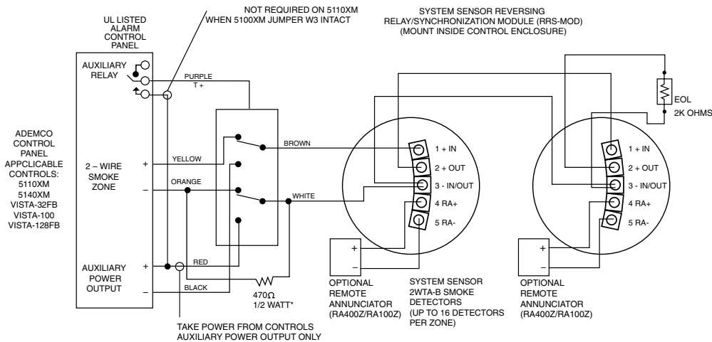
FIGURE 6. CONNECTING 2WTA-B SMOKE DETECTORS TO ADEMCO CONTROLS USING RRS-MOD MODULE TRIGGERED FROM AUXILIARY RELAY:
