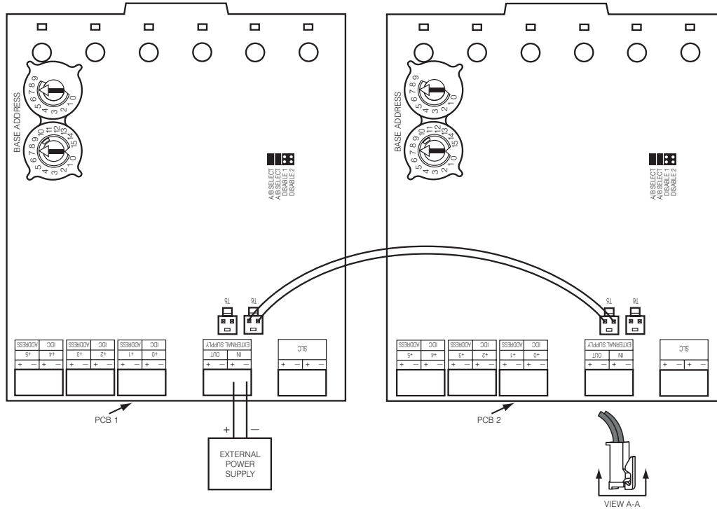
FIGURE 10. EXAMPLE OF MULTIPLE BOARDS SHARING SAME EXTERNAL SUPPLY
