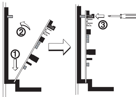
FIGURE 5. INSTALLATION OF REAR MODULE ONLY, METHOD ONE
