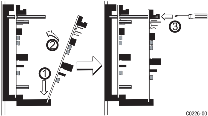
FIGURE 6B. INSTALLATION OF MMF-300-10A MODULE IN FRONT CHASSIS POSITION
