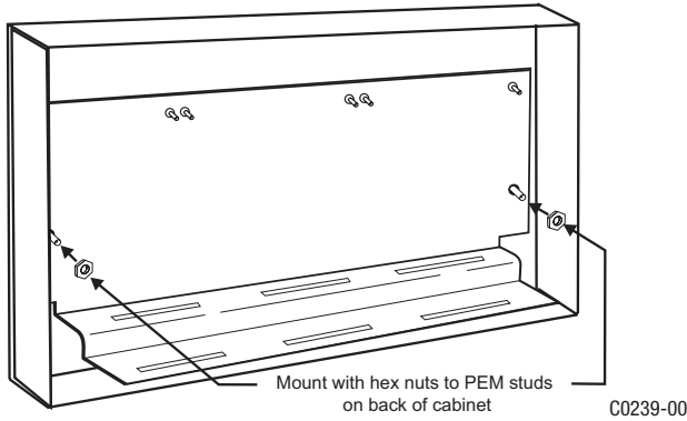
FIGURE 4. MOUNTING THE CH-6 CHASSIS
