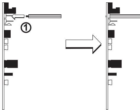
FIGURE 6A. INSTALLATION OF MMF-300-10A MODULE IN A REAR CHASSIS POSITION, METHOD TWO
