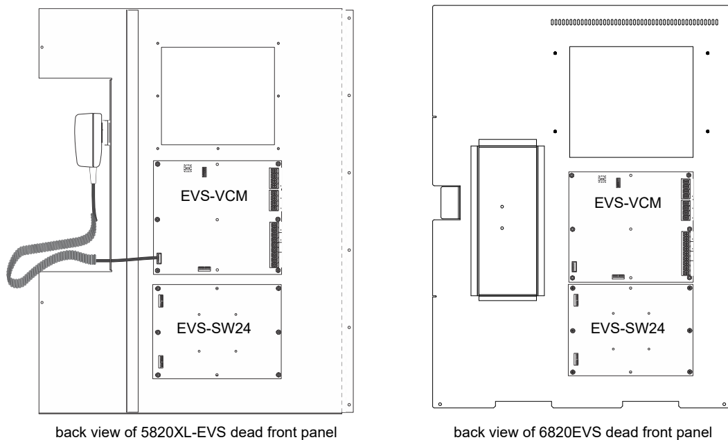
Figure 1 EVS-SW24 Mounting Locations
