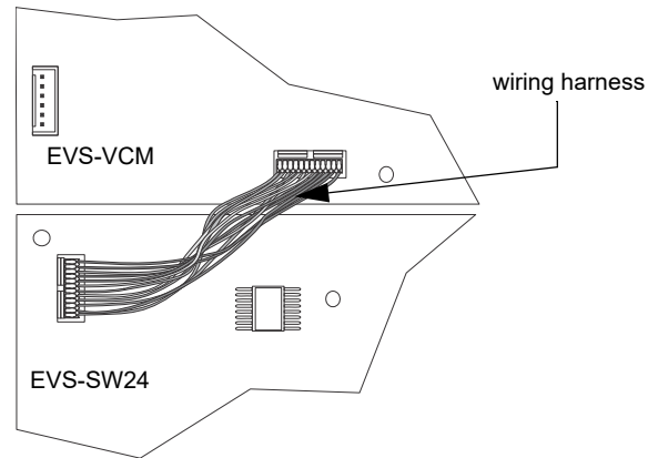
Figure 2 Connection for EVS-VCN to EVS-SW24
