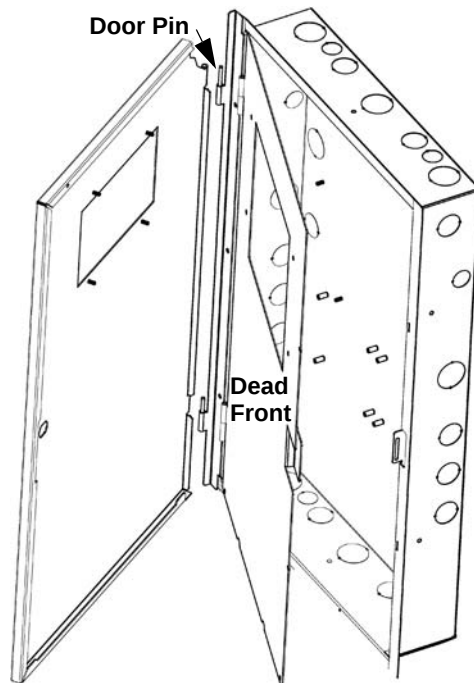
Figure 3: EVS-LOC Cabinet
