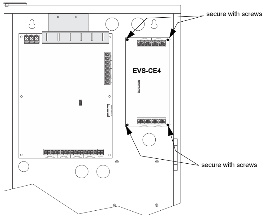
Figure 1 Mounting the EVS-CE4
