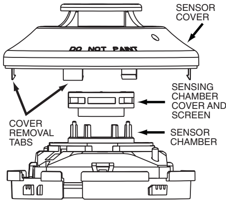
FIGURE 10. DETECTOR SENSOR EXPLODED VIEW:
