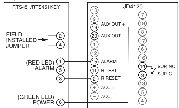
FIGURE 13. WIRING DIAGRAM FOR D4120 TO RTS451/RTS151/RTS-451KEY/RTS151KEY:
