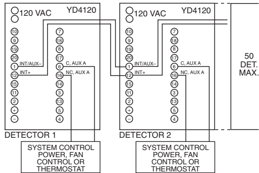
FIGURE 8. MULTIPLE FAN SHUTDOWN (INTERCONNECTION OF D4120'S):
