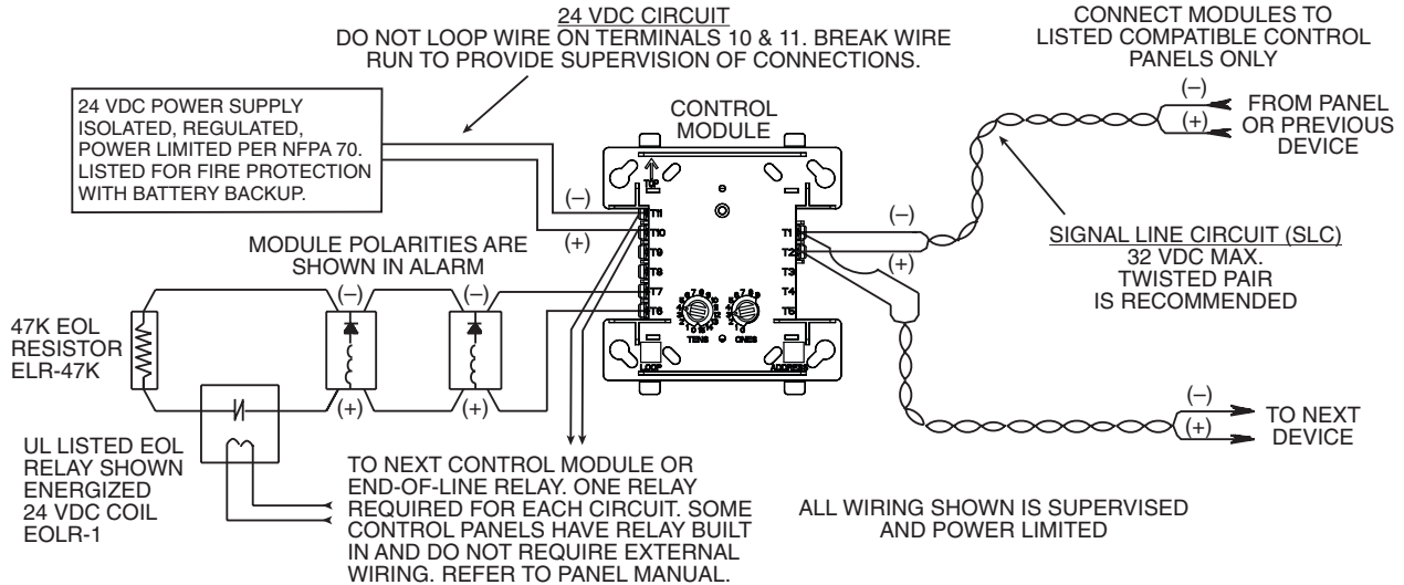
FIGURE 3. TYPICAL NOTIFICATION APPLIANCE CIRCUIT CONFIGURATION, NFPA STYLE Y (CLASS B):
