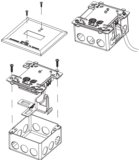
FIGURE 2A. MODULE MOUNTING WITH BARRIER: FIGURE 2B:
