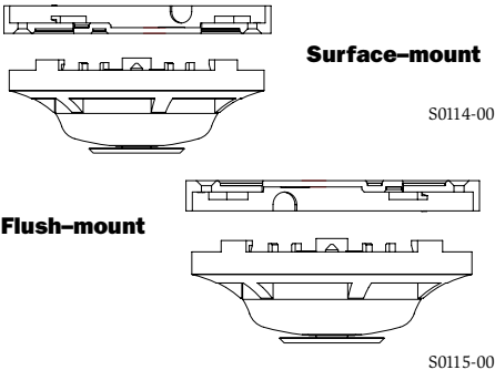
Figure 2. Reversible Mounting Bracket:
