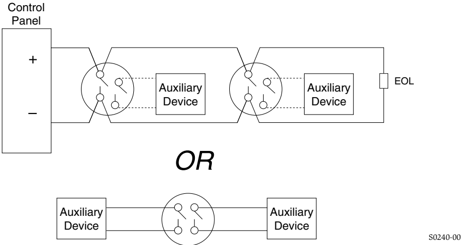
Figure 4. Wiring Diagram – Dual Circuit Models:
