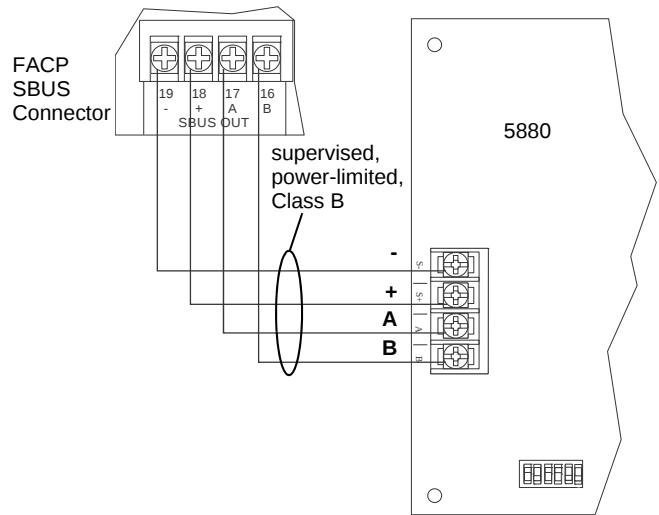
Figure 2 5880 Connection to the FACP
