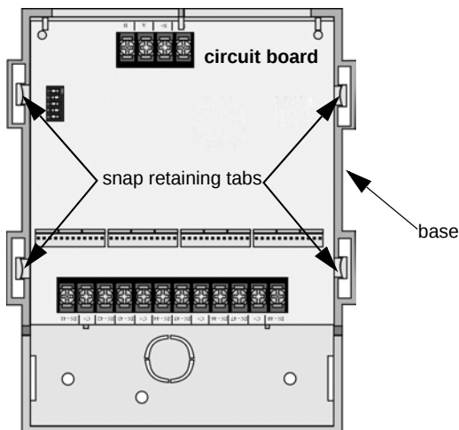
Figure 1 5880 Circuit Board and Plastic Base
