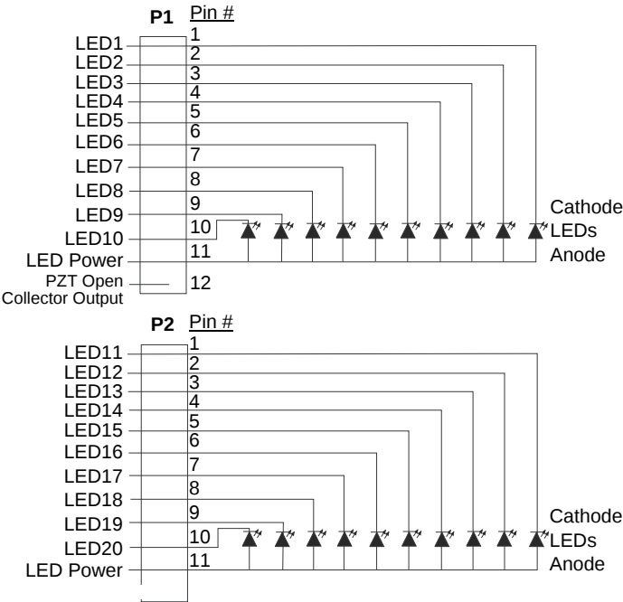
Figure 3 5880 LED Outputs
