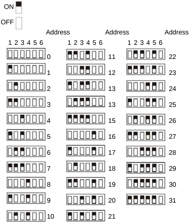
Figure 5 DIP Switch Settings
